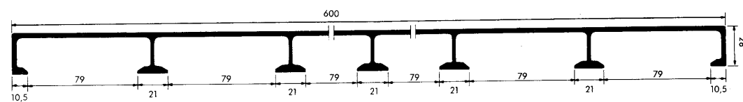
AS34895 Δ 4,90 kg/m code 530609 6,025 m
